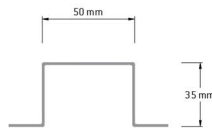
Typical intermediate top hat profile
