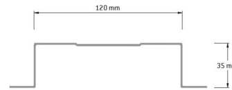
Typical joint top hat profile located at panel vertical joints
