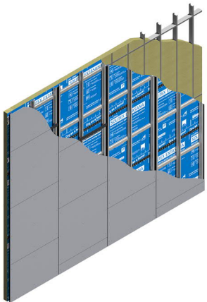
Isometric view of double layer top hat construction
