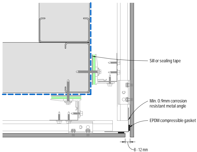
Figure 25: External corner
