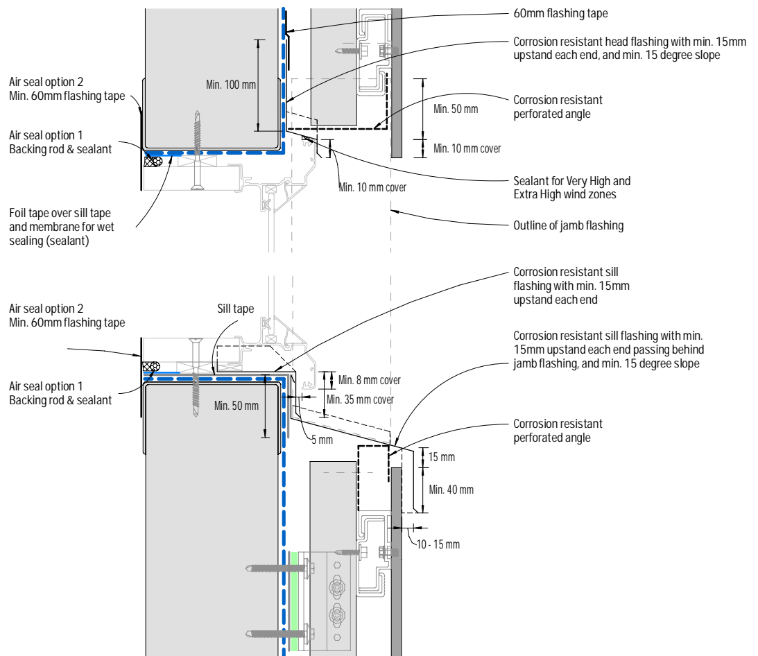
Figure 10: Recessed window - Head and sill
