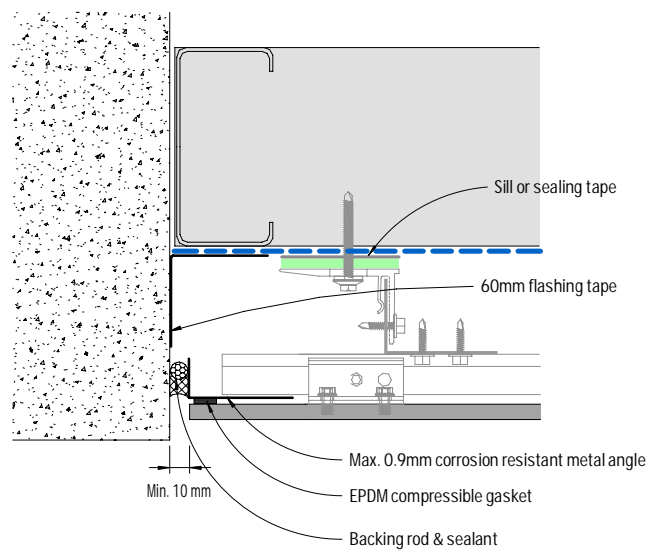
Figure 26: Abutment
