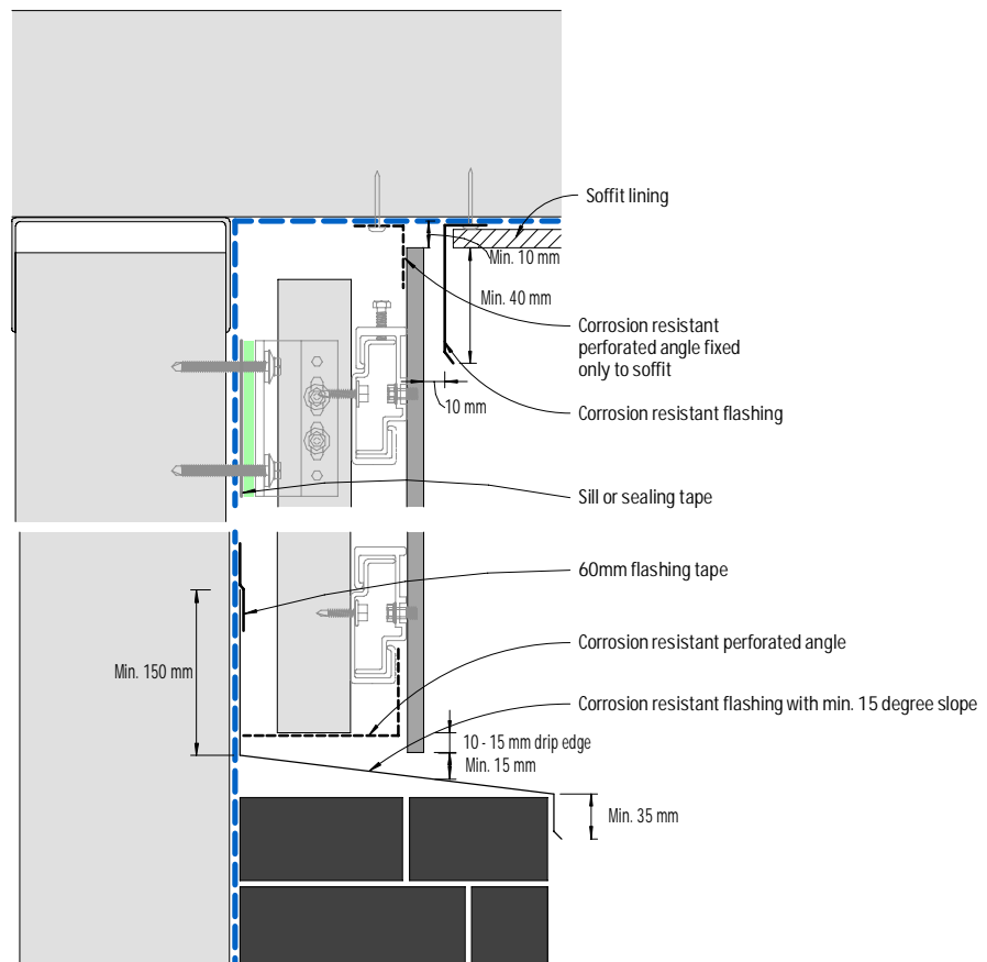
Figure 22: Junction with other materials, eaves or the like - recessed detail
