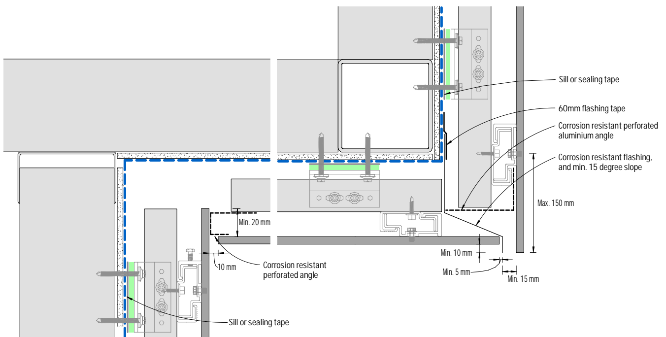
Figure 19: Soffit junction
