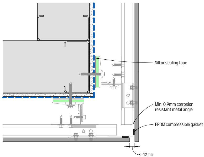
Figure 27: External corner
