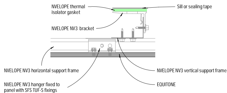
Figure 5: Intermediate panel fixings connection
