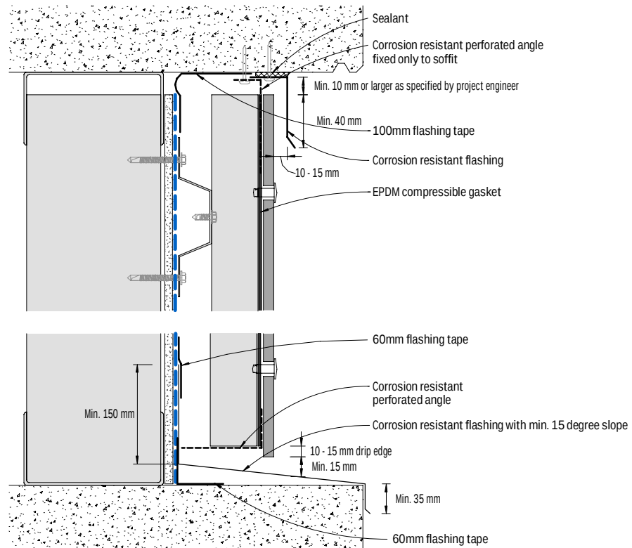
Figure 28: Exposed concrete slab or beam - Cladding recessed
