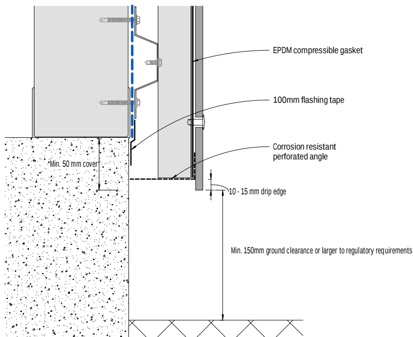
Figure 20: Base detail
