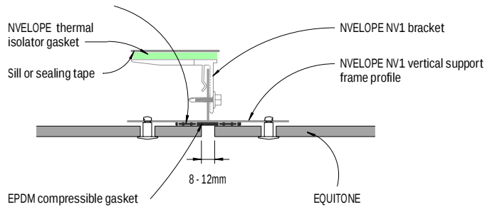
Figure 5: Vertical joint - Detail 1
