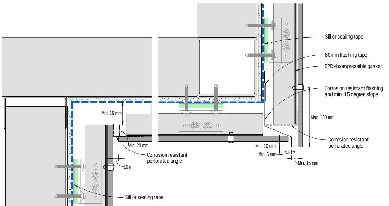
Figure 21: Soffit junction
