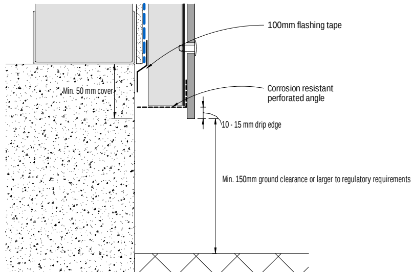
Figure 22: Base detail
