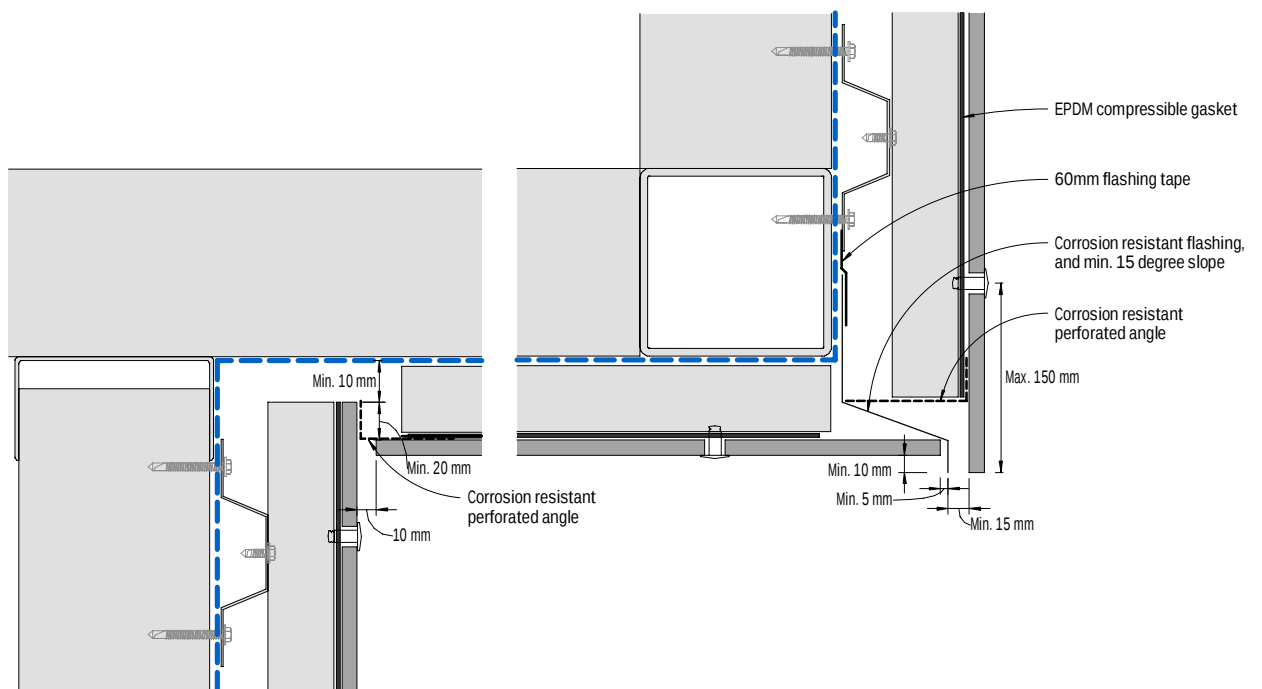
Figure 19: Soffit junction
