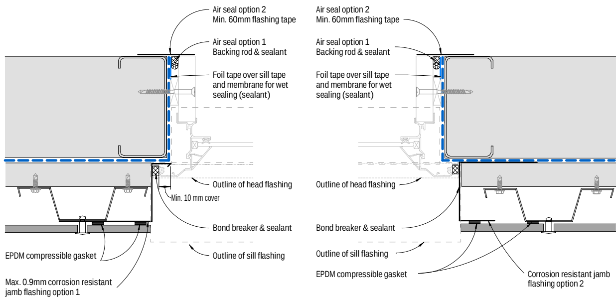
Figure 13: Recessed window jamb - Option 1
