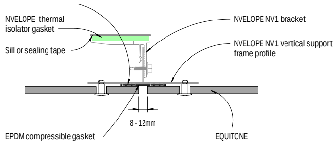
Figure 3: Vertical joint - Detail 1
