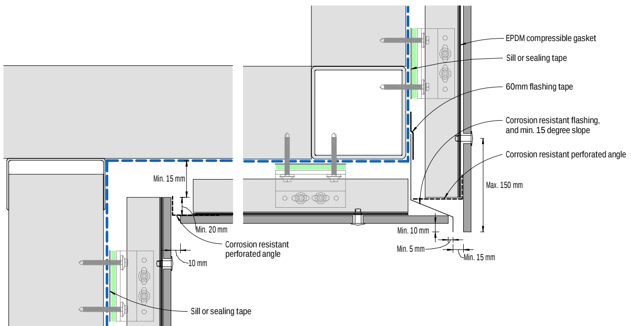
Figure 19: Soffit junction
