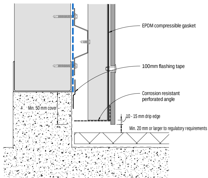
Figure 21: Base detail - Covered area
