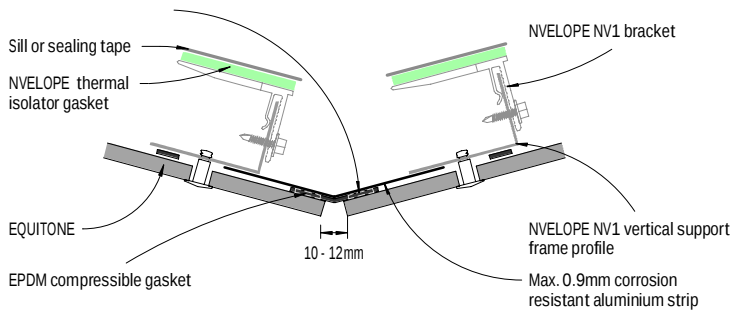
Figure 5: Vertical joint - Detail 3
