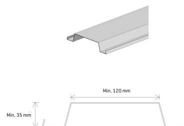
Typical joint top hat profile located at panel vertical joints
